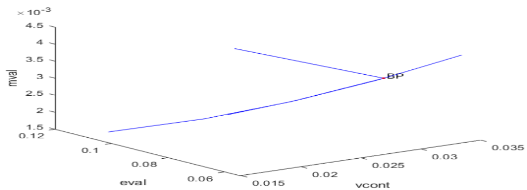
Fig. 5 Bifurcation Diagram (Model 2)
